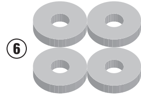
Hole Ø8,5mm/ External Ø24mm/ H.5mm
